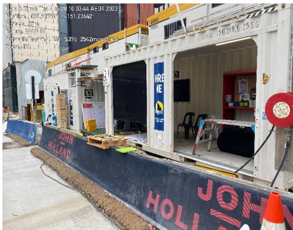
Nurse station adjacent to temporary driveway. Covered drain surrounded by a coir log Coir logs lining temporary driveway to mitigate dirty water runoff beneath the concrete divider. adjacent to site temporary driveway from Botany Road.
